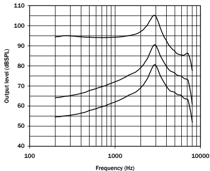
OSPL Curves @ 50/60/90 dB SPL Input
