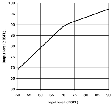
Input/Output Function @ 2000 Hz
